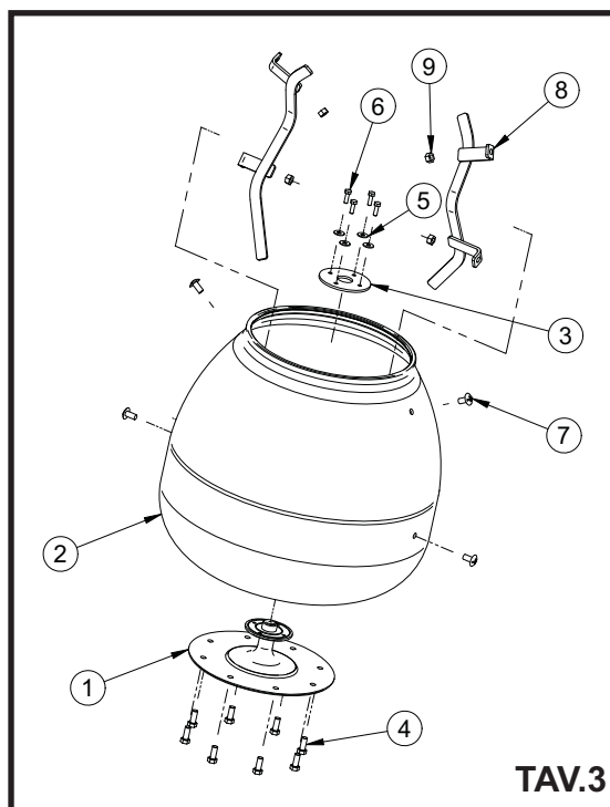
TAV.3 KIT VASCA IN PLASTICA - KIT CUVE PLASTIQUE - KIT PLASTIC DRUM - KIT PLASTIK RÜHRARM - KIT TAMBOR PLASTICO
